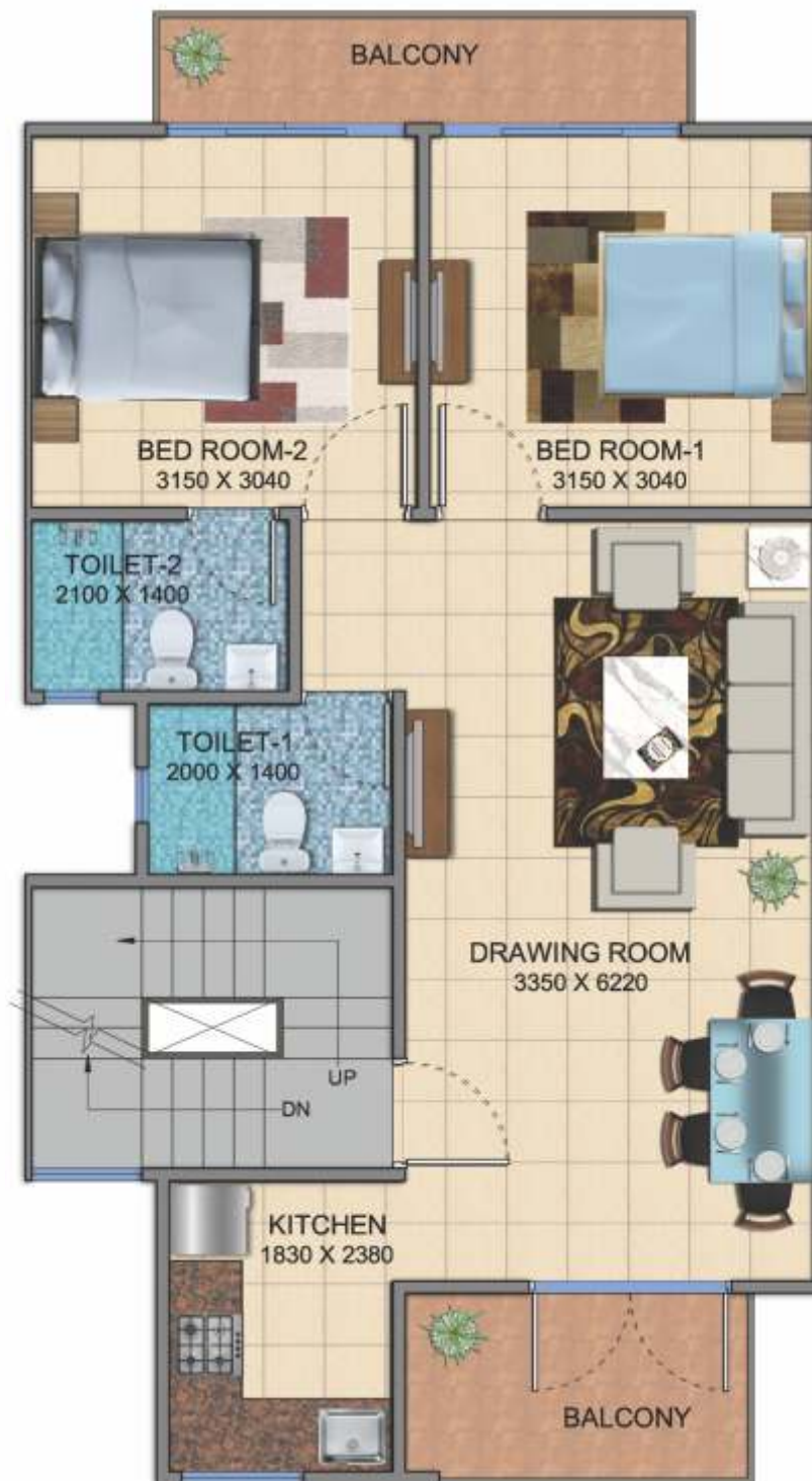
2 BHK (TYPICAL) FIRST AND SECOND FLOOR
