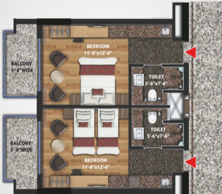
SUITE FLOOR PLAN SALEABLE AREA - 435 SQ.FT.
